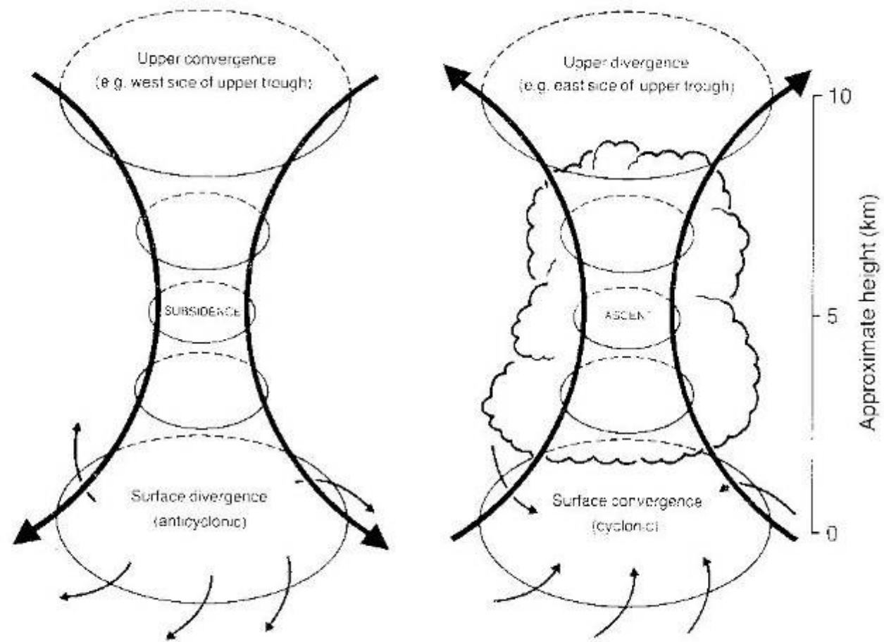
Fig. 4.6 A schematic illustration indicating patterns of convergence and divergence at the surface and in the upper atmosphere are linked with vertical motions.
