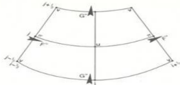
Figure 7.9 The grid centered on a u point.
