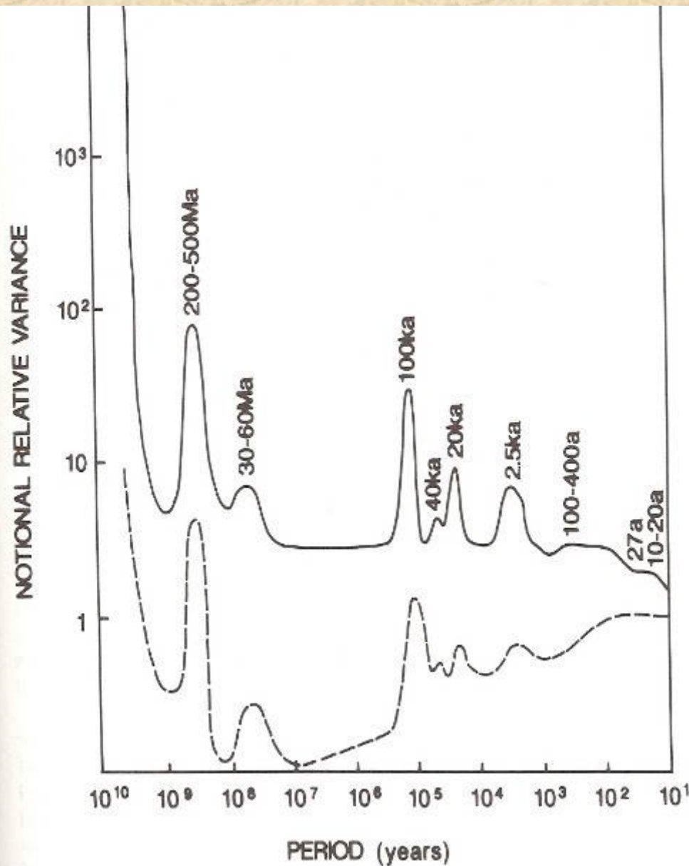
Figure 1.1 Notional estimates of the relative variance of climate over all periods of variation, from 4.5 Ga to 10 a (solid line). The strongest periodic components of variation are labelled. The relative variance for periods in excess of 1 Ga is, in effect, meaningless, since the age of the Earth is insufficiently long for several cycles to have occurred. The dashed line attempts to show the geographical scale of climate variations: the area below it represents the contribution to the total variance of climate processes operating on a spatial scale of less than 1000 km. (From Mitchell, 1976.)
