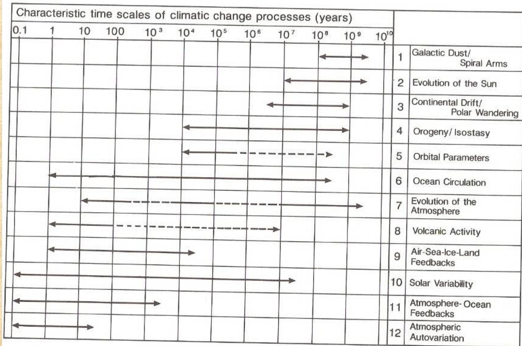
Figure 1.2 Major mechanisms of climate change and their time scales of operation. (Based on Wigley, 1981.)
