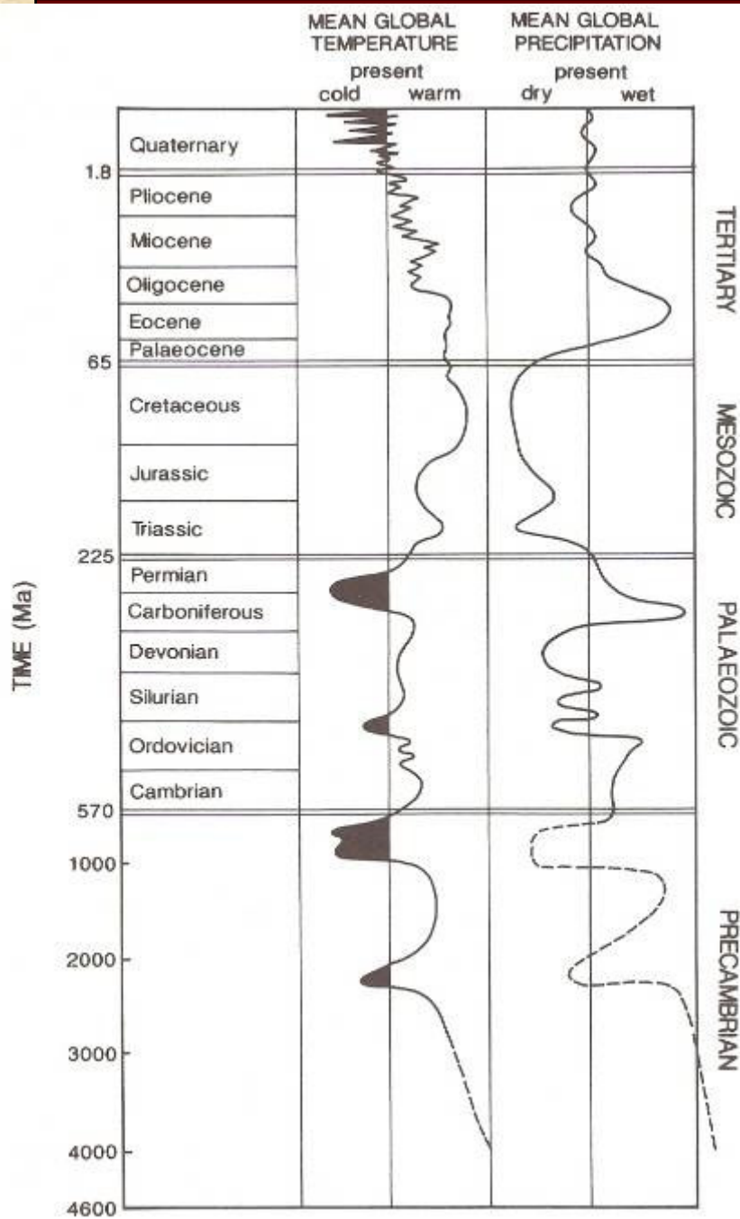
Figure 1.3 Generalized temperature and precipitation history of the Earth. The curves indicate relative departures from present global means. Periods colder than today are shaded. Dashed lines indicate periods of sparse data. Note that the time scale is progressively expanded from bottom to top. (From Frakes, 1979.)
