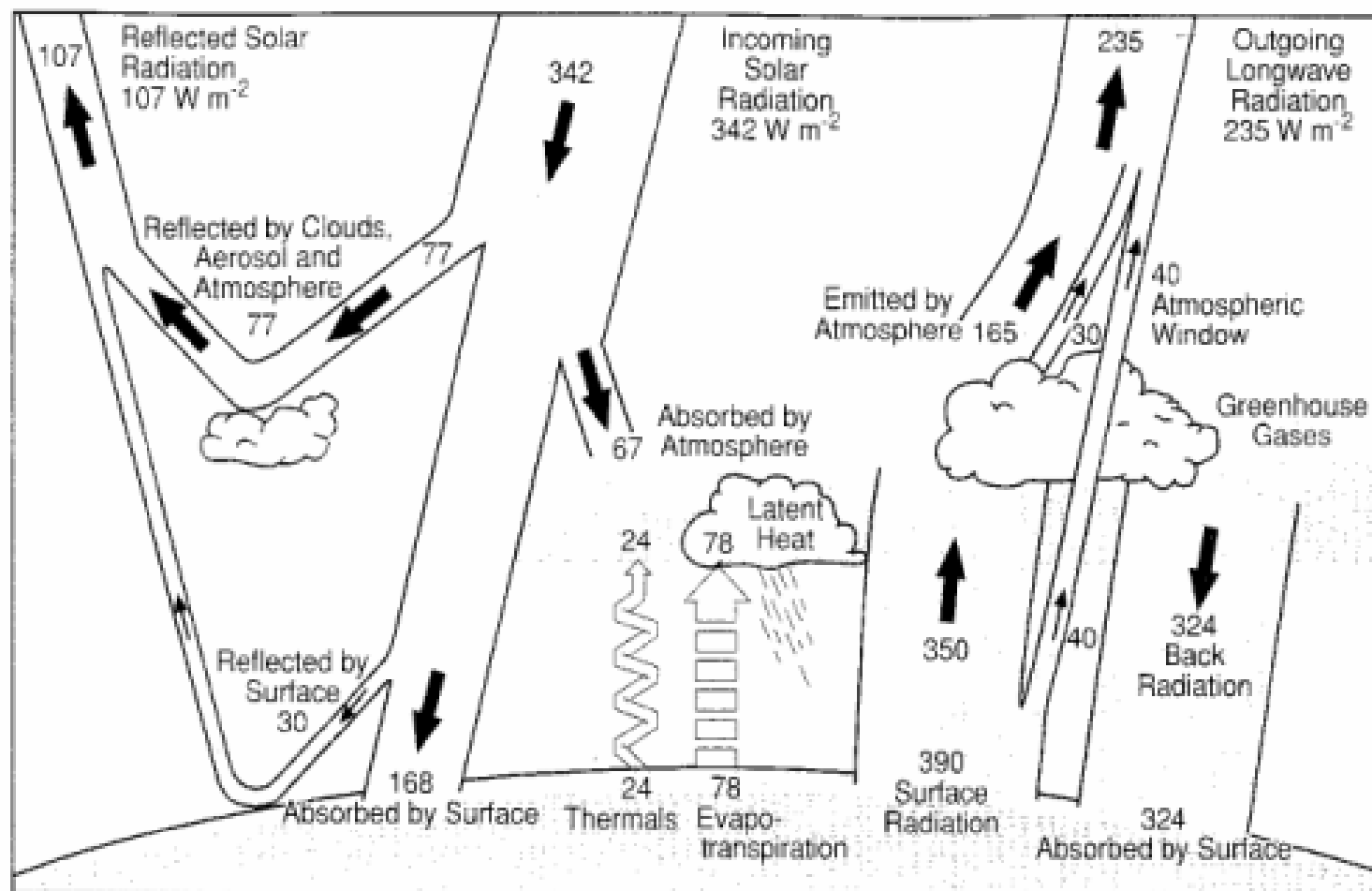
Figure 1.3: The Earth's radiation and energy balance. The net incoming solar radiation of 342 \text{ W m}^{-2} is partially reflected by clouds and the atmosphere, or at the surface, but 49% is absorbed by the surface. Some of that heat is returned to the atmosphere as sensible heating and most as evapotranspiration that is realised as latent heat in precipitation. The rest is radiated as thermal infrared radiation and most of that is absorbed by the atmosphere which in turn emits radiation both up and down, producing a greenhouse effect, as the radiation lost to space comes from cloud tops and parts of the atmosphere much colder than the surface. The partitioning of the annual global mean energy budget and the accuracy of the values are given in Kiehl and Trenberth (1996).
